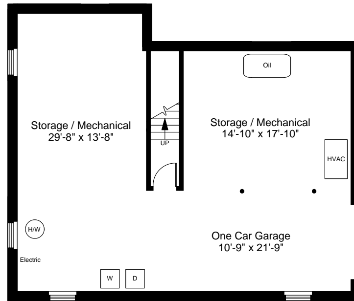
Guest House - Basement Floor Plan Ceiling Height = 7'-10"
