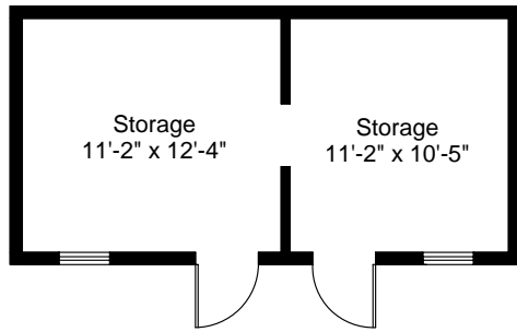
Storage Shed Floor Plan
