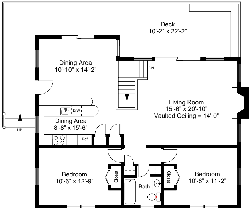
Guest House - First Floor Plan Ceiling Height = 8'-2"
